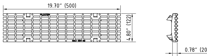
C250kN MW29/6: GJS 17010106
